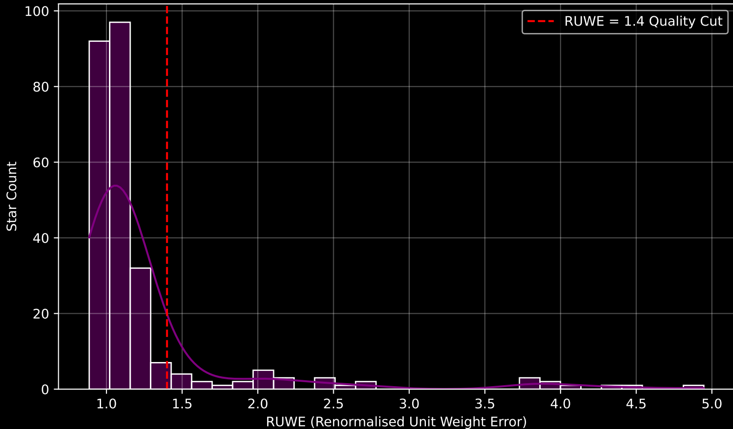
GALAH DR4 Field [9274] RUWE Distribution (n= 260)
