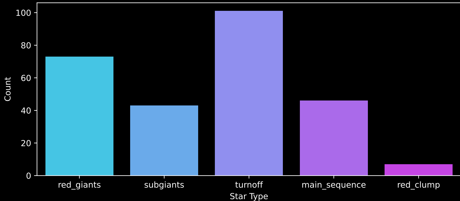
GALAH DR4 Field: [9274] Count plot of Star Type
