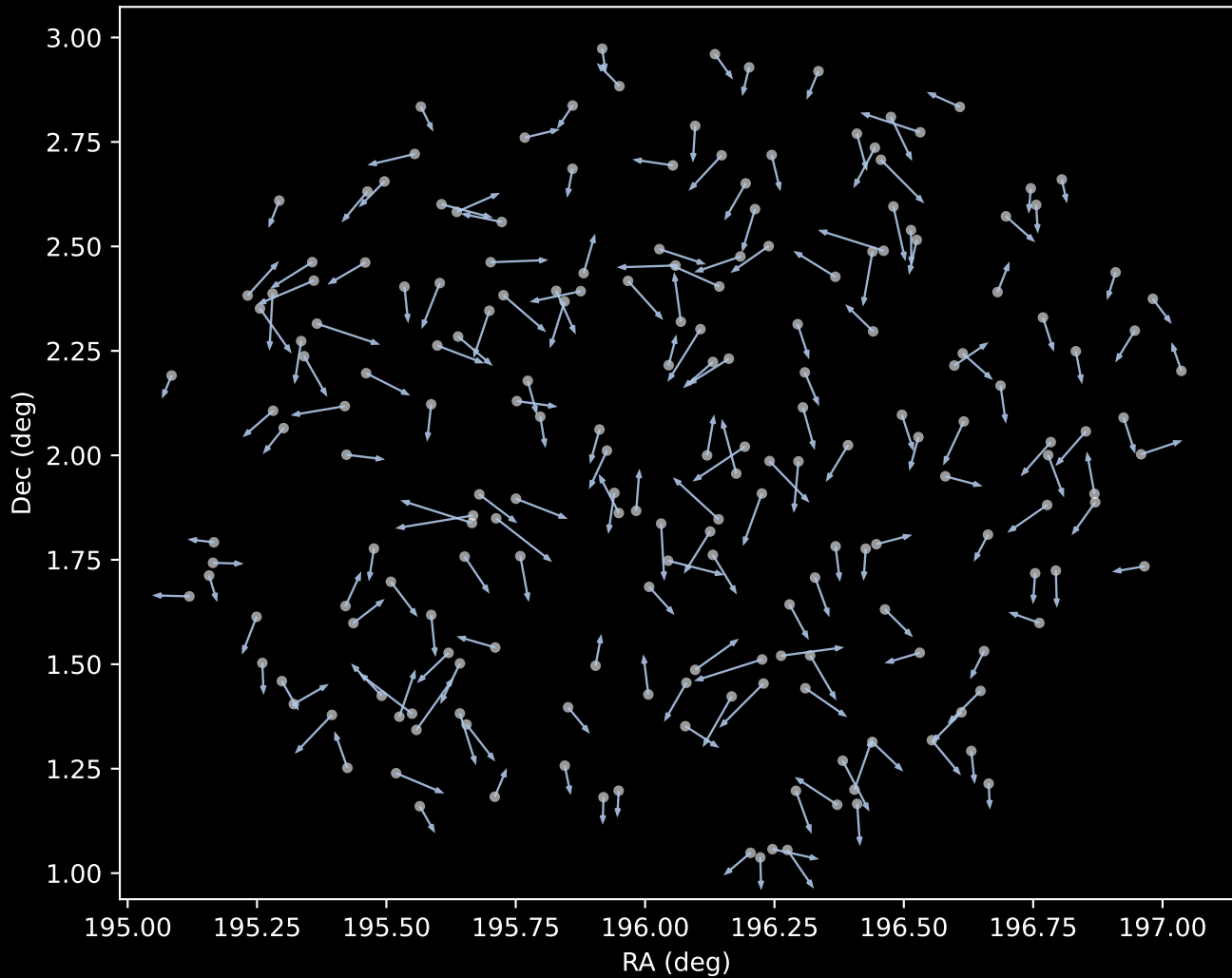
GALAH DR4 Cluster 1 Proper Motion Vectors (n=200)
